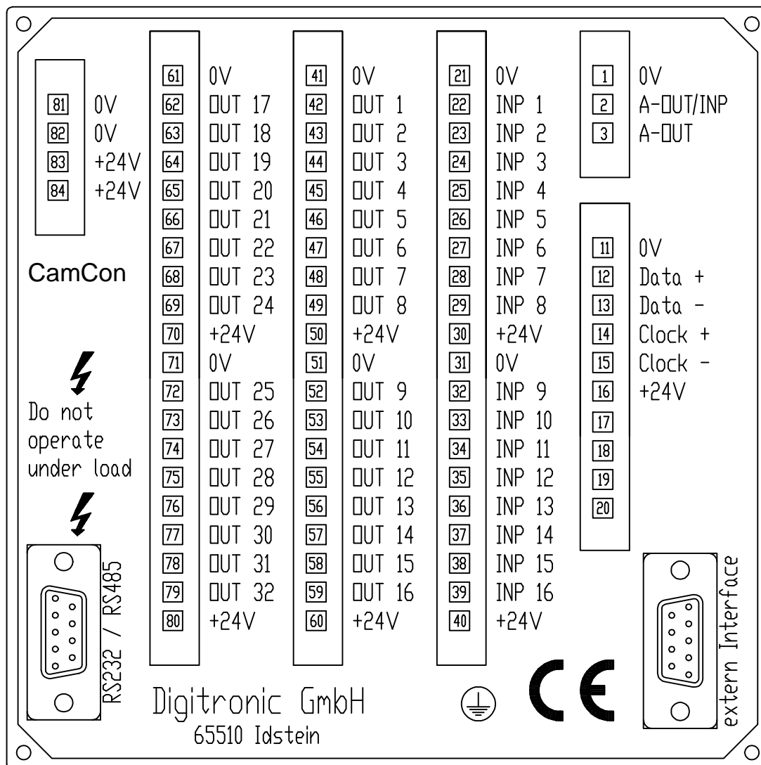
Fig.: Backview of the CamCon with pin allocation
