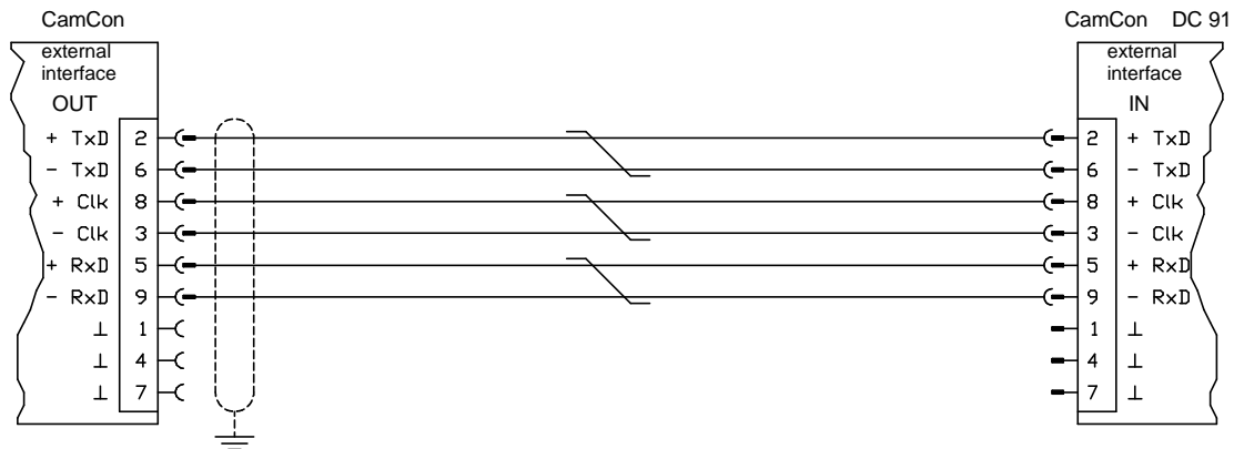
Connection cable CamCon DC91/IO
