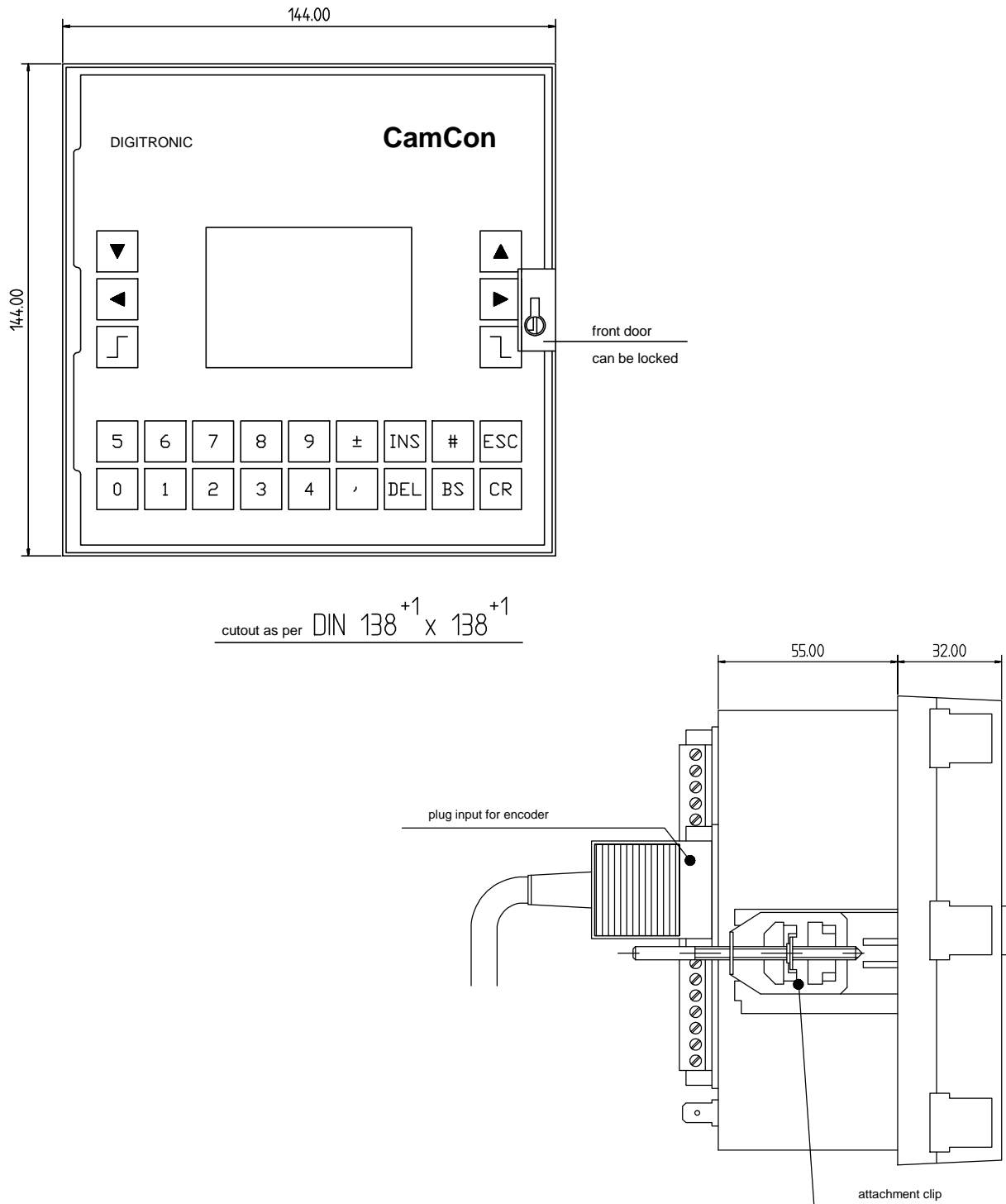
Fig.: Drawing to aid the installation of CamCon
